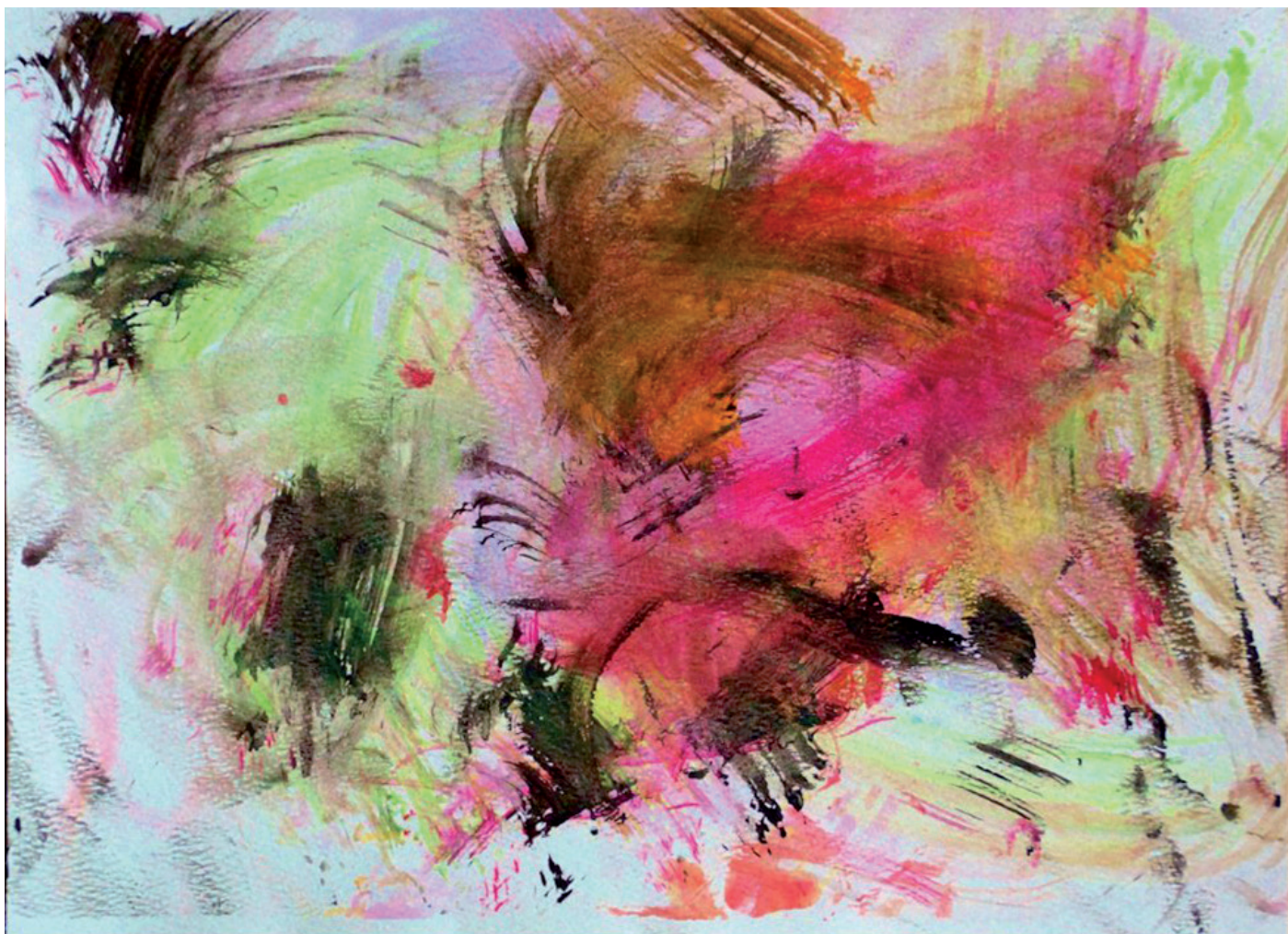
Bradford Smith
